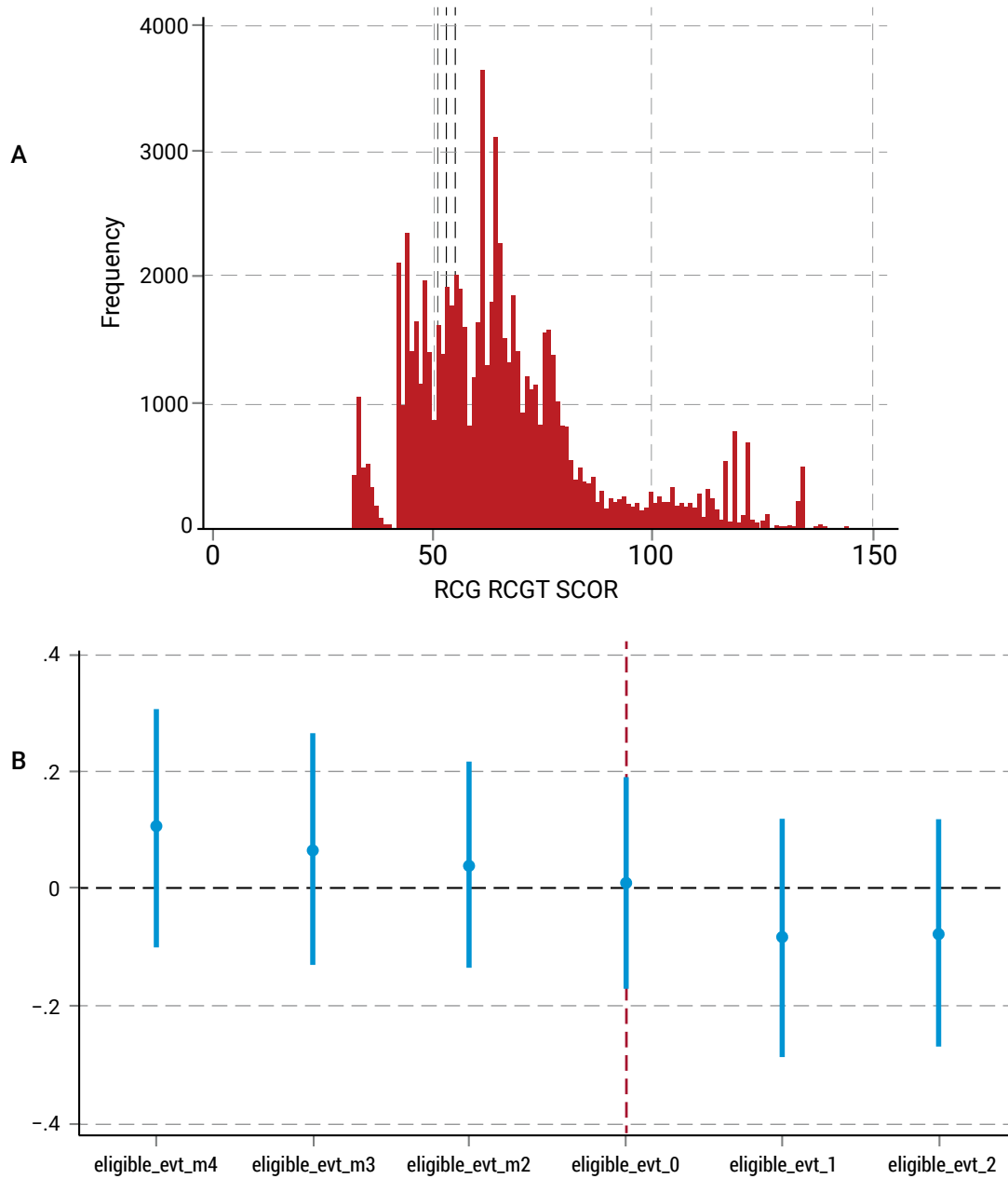
FIGURE 1 Fixed-effects RD-DID validity check: distribution of LTCI assessment scores and event study
